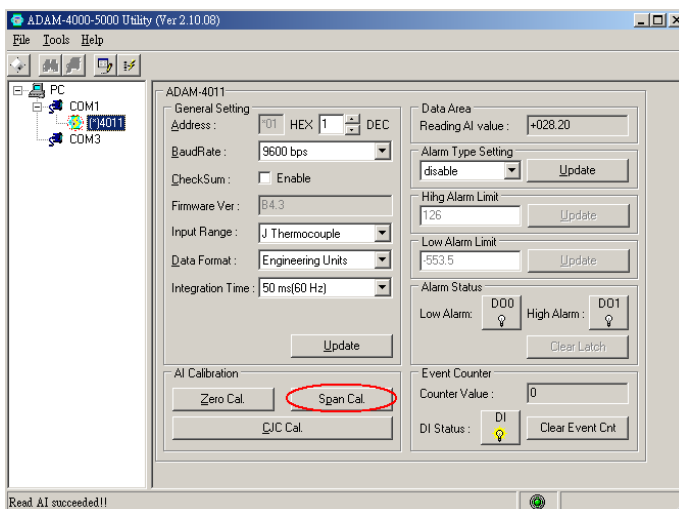
Figure 8-3 Span Calibration
