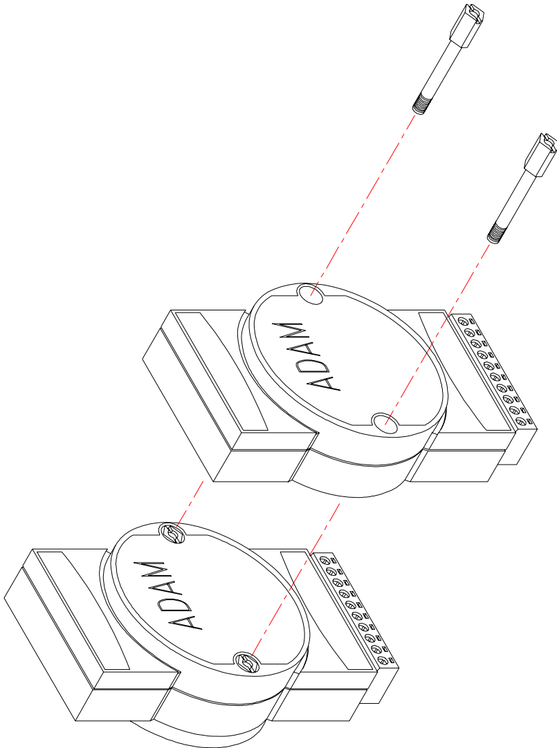
Figure C-6 Piggyback Stack
