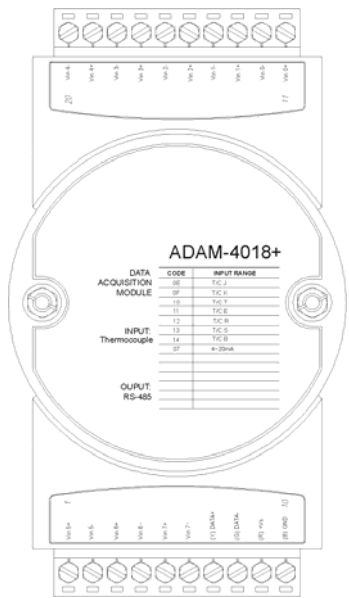
Figure 3-29 ADAM-4018+ 8-ch. thermocouple input module
