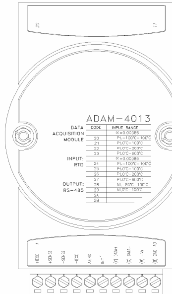
Figure 3-15 ADAM-4013 RTD Input Module
