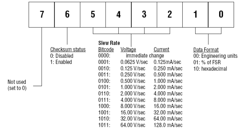
Figure 6-1 Data format for FF (8-bit parameter)
