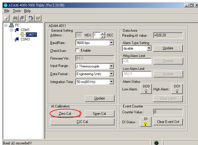
Figure 8-2 Zero Calibration
