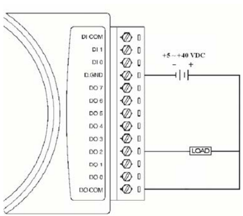
Figure 3-53 ADAM-4055 Digital Output Wiring Diagram
