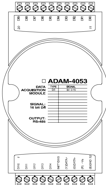
Figure 3-49 ADAM-4053 16-channel Digital Input Module
